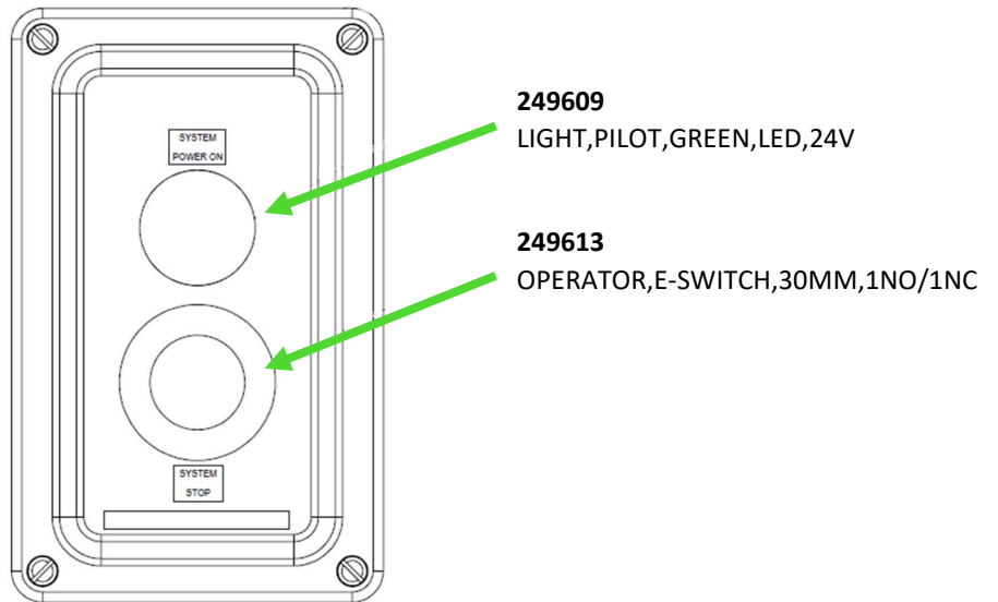
Figure 1. System Stop Box Layout
